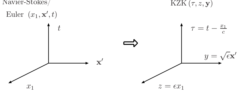
Figure 2: Paraxial change of variables for the profiles U(t - x_1/c, \varepsilon x_1, \sqrt{\varepsilon} x') .
