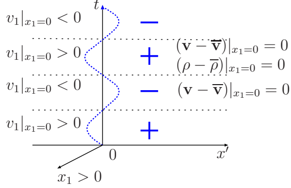
Figure 3: Periodic subsonic inflow-outflow boundary conditions for the Navier-Stokes system.
