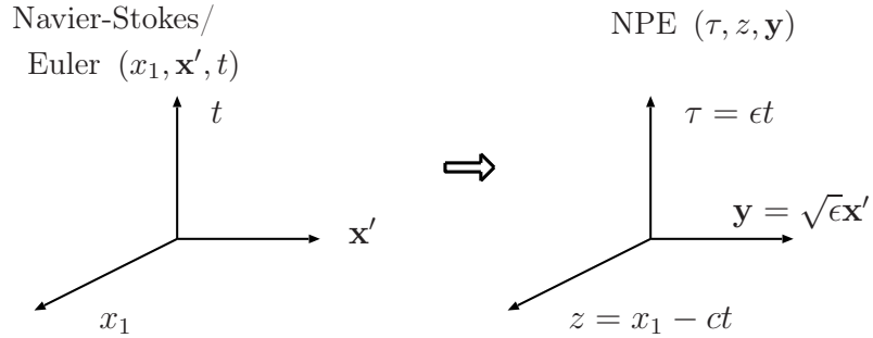
Figure 4: Paraxial change of variables for the profiles U(\varepsilon t, x_1 - ct, \sqrt{\varepsilon} \mathbf{x}') .
