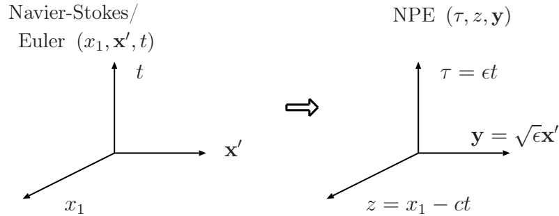
Figure 3: Paraxial change of variables for the profiles U(\varepsilon t, x_1 - ct, \sqrt{\varepsilon} x') .
