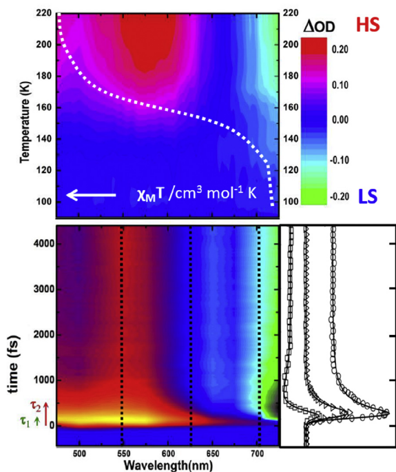
Fig. 7. Thermal (top) and photoinduced change (bottom) of optical density after a femtosecond excitation in nanocrystals of [Fe(3-MeO-SalEen) 2 ]PF 6 . The kinetic traces reveal the HS spectral fingerprints in the time domain within 1 ps. Adapted from Ref. [50].
