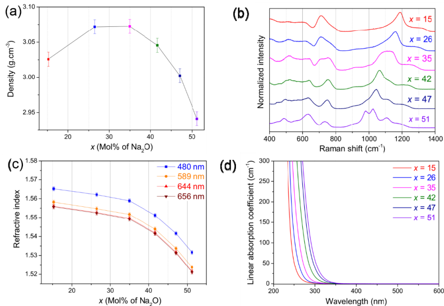
Fig. 2. Properties of the \text{GPN}_x\text{:Ag} series as function of the \text{Na}_2\text{O} content x (a) Density (b) Normalized raw Raman spectra (c) Refractive indices measured at 480, 589, 644 and 656 nm and (d) Linear absorption coefficient spectra in UV-visible region. Lines are guides for the eyes for (a) and (c).
