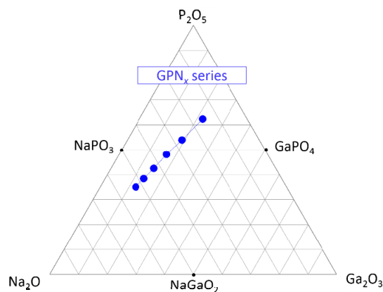
Fig. 1. Ternary diagram of P_2O_5 - Ga_2O_3 - Na_2O with investigated compositions (blue dots) (note all compositions contain 2 Mol% of silver oxide in addition, corresponding to the GPN_x:Ag series)
