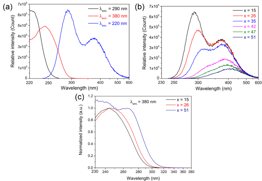
Fig. 3. (a) Excitation and emission spectra of \text{GPN}_{15}:\text{Ag} glass (b) Emission spectra of both isolated \text{Ag}^+ ions and \text{Ag}^+-\text{Ag}^+ dimers with a selective excitation of the isolated \text{Ag}^+ ions at 220 nm and (c) Selective excitation spectra of \text{Ag}^+-\text{Ag}^+ dimers for an emission at 380 nm in \text{GPN}_x:\text{Ag} series. The inset shows the normalized excitation spectra of \text{Ag}^+-\text{Ag}^+ dimers for an emission at 380 nm in \text{GPN}_x:\text{Ag} series.
