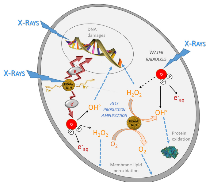
Fig. 3. Schematic illustration of radiotherapy enhancement by metal-based nanoparticles. When encounter the cell, incident X-photons beam induce excitations and ionizations of intracellular components, causing direct effects such as DNA damages ( e.g. DNA simple- and double-strand breaks, DNA-protein crosslinks), and the water radiolysis leading to ROS production. Reactive oxygen species in turn alter cellular macromolecules inducing protein oxidation, membrane lipid peroxidation and indirect DNA damages. In presence of high-Z nanoparticles, the interactions between X-rays and nanoparticles result in an amplified production of secondary electrons and ROS, contributing to enhanced cytotoxic effects on irradiated cells.
