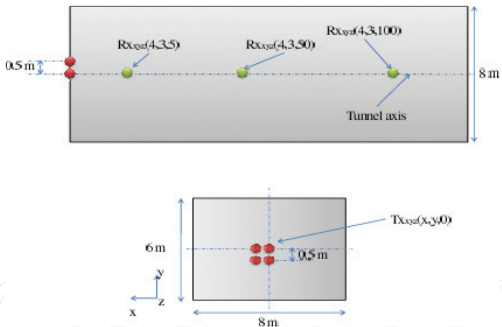
Figure 7. Time focusing simulation setup.
