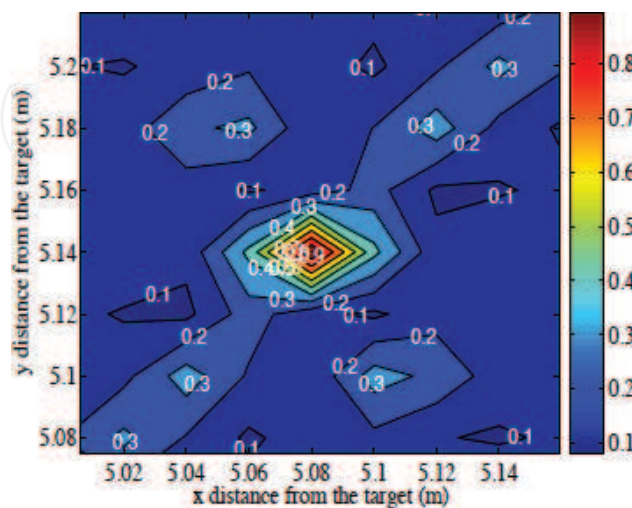
Figure 9. Spatial focusing gain in the SISO-TR case.
