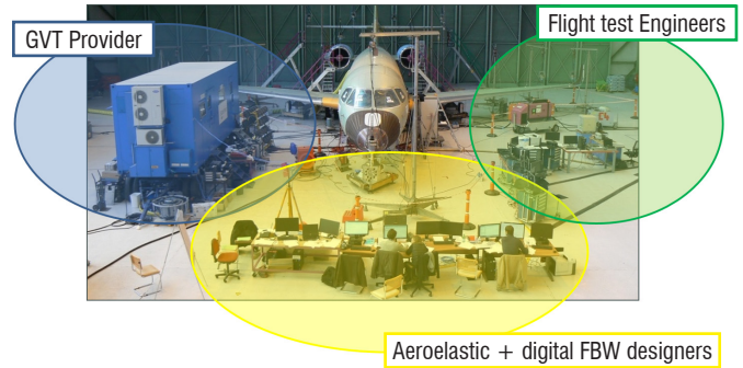
Figure 28 – Ground Vibration Test typical collaborative installation
