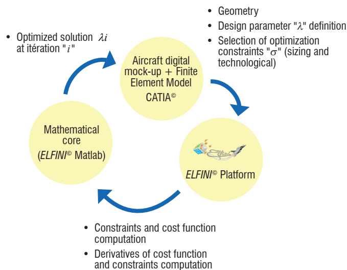
Figure 19 – Dassault Aviation global aero-structural optimization process
