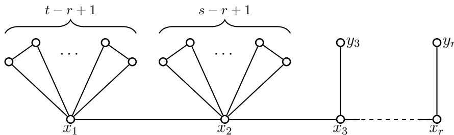
Figure 1: Graph G_{r,s,t}
