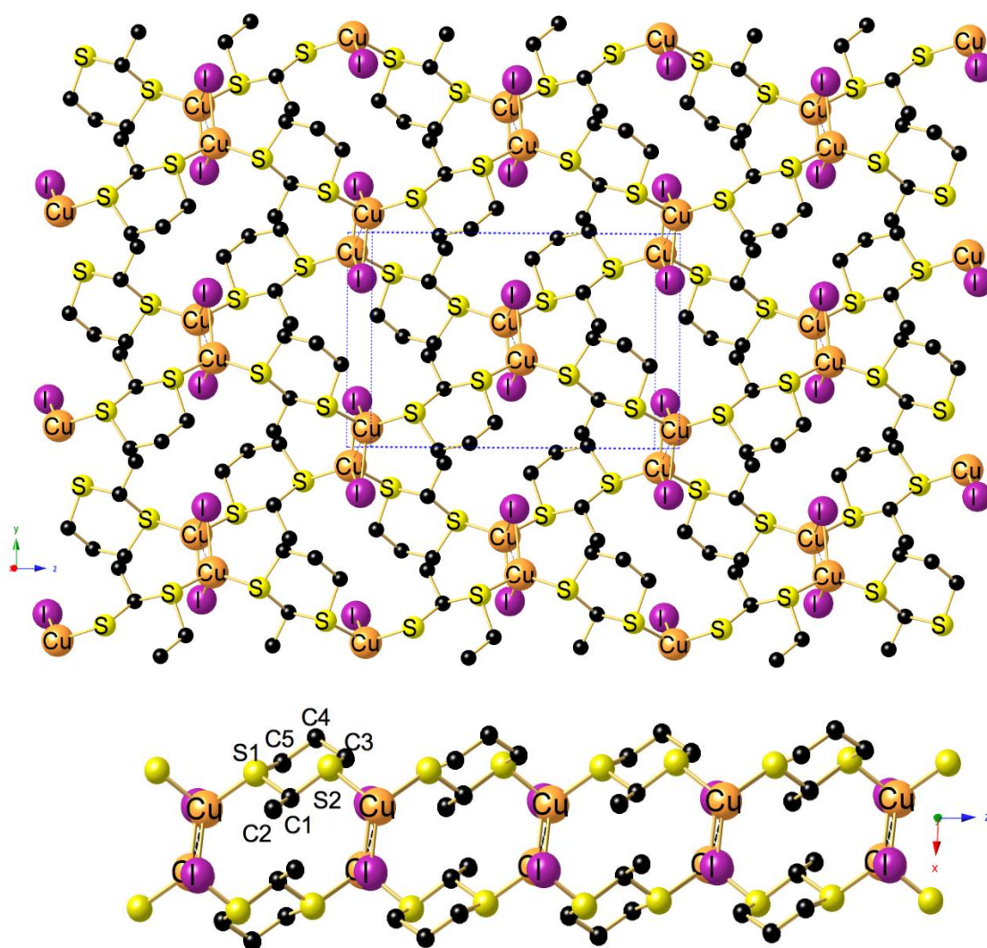
Figure 2. (Top) View on the y,z plane of the 2D network of [\{\text{Cu}(\mu_2\text{-I})_2\text{Cu}\}(\mu_2\text{-L2})_2]_n CP2 . Selected bond lengths (Å) and angles (°): Cu····Cu# 2.7664(6), Cu–I 2.6162(5), Cu–I#
