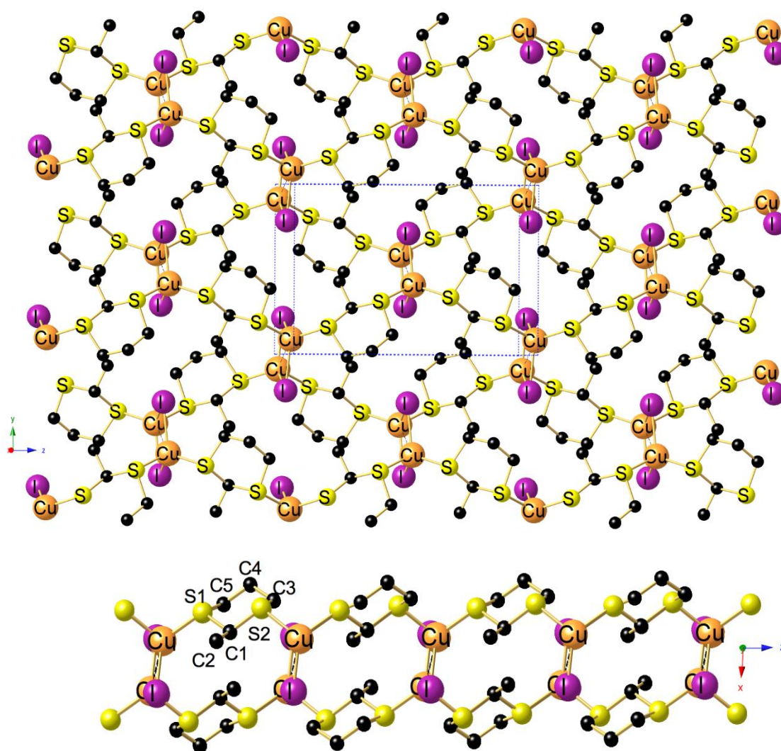
Figure 2. (Top) View on the y,z plane of the 2D network of [\{\text{Cu}(\mu_2\text{-I})_2\text{Cu}\}(\mu_2\text{-L2})_2]_n CP2 . Selected bond lengths (Å) and angles (°): Cu···Cu# 2.7664(6), Cu–I 2.6162(5), Cu–I#
