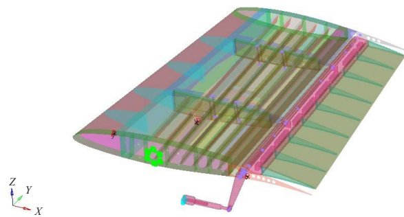
Figure 7 – CRIAQ MDO 505 morphing wing model
