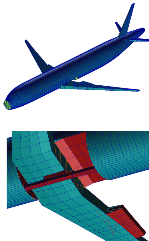
Figure 8 – Full aircraft finite-element model and detailed coupling region of the wing-fuselage intersection
