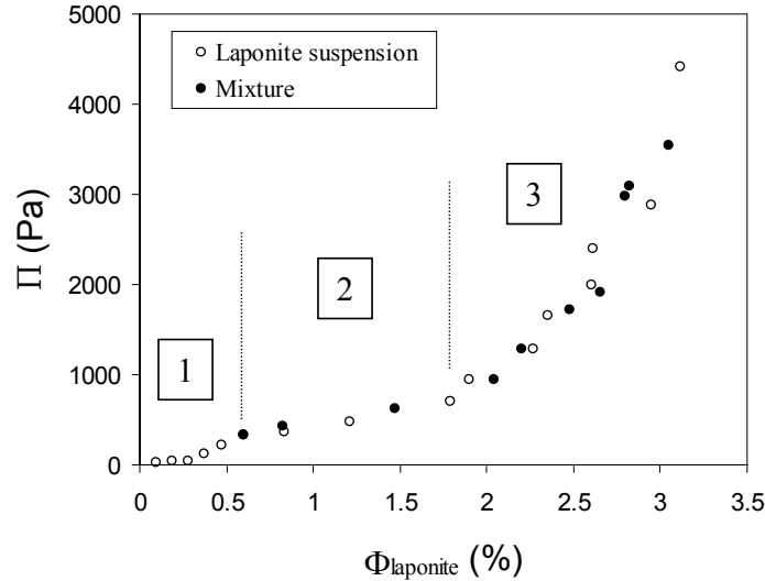
Fig. 7: Experimental state isotherm curve \Pi vs. \Phi for pure laponite suspensions in a \text{Na}_3\text{Cit} solution ( 2.5 \cdot 10^{-3} \text{ mol.L}^{-1} ) at pH 10 (open dots) and for laponite doped with maghemite probes in the same chemical conditions (filled dots). The dotted lines separate the three characteristic domains of the equation of state considered in the text (before, along and after the pseudoplateau) [14].
