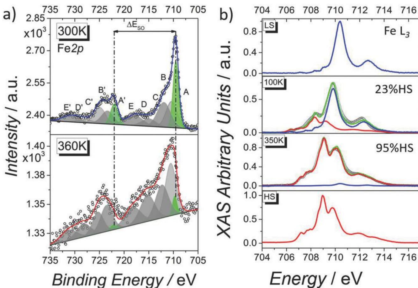
Figure 2 : a) Temperature dependence of the Fe2p XPS spectra evidencing thermal SCO behavior for 6.7 nm thick films of 1 on 76 Au and b) temperature evolution of the normalized Fe L 3 edge XAS spectra of a thermally evaporated 6.7 nm thin film of 1
