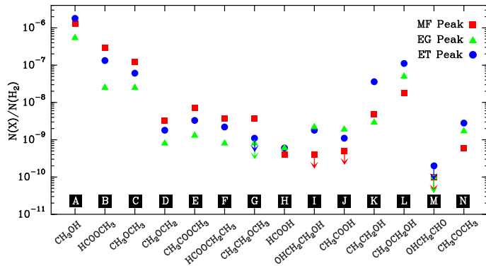
Fig. 2. Abundances of complex O-bearing species in Orion KL.
