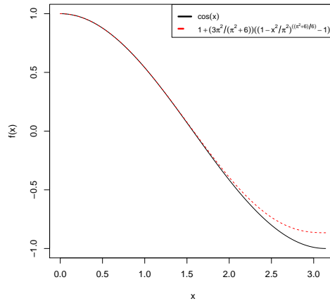
Figure 2: Graphs of the functions in (3.3) for x \in (0, \pi) .
