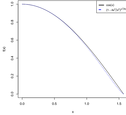
Figure 1: Graphs of the functions in (3.1) for x \in (0, \pi/2) .
