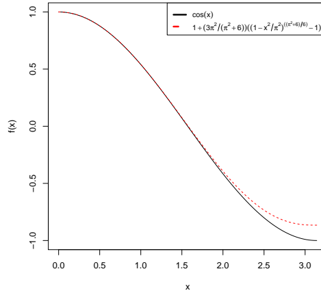
Figure 2: Graphs of the function and the bound in (3.3) for x \in (0, \pi) .
