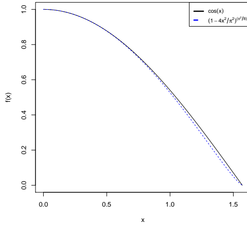
Figure 1: Graphs of the function and the bound in (3.1) for x \in (0, \pi/2) .
