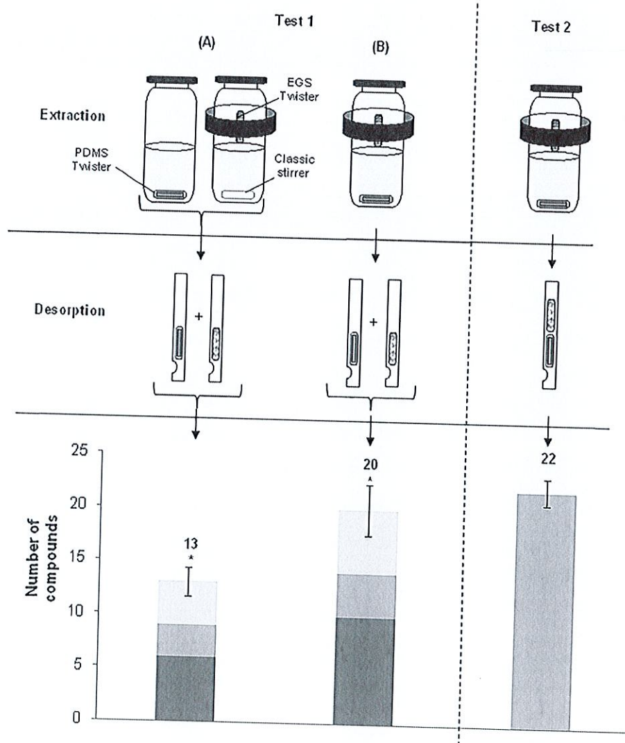
Fig. 4. Schema and results of separate or simultaneous extraction and desorption. The histograms are stacked with the compounds found with EGS twister in dark grey, while those found with PDMS twister are in light grey; in grey, molecules extracted with these two stir bars are visible. The significant difference between tests is indicated by a star. Errors bars indicate the standard deviation of the identification of the compounds in the three independent replicates. "Test 1" compares the efficiency of separate extraction (two vials/two bars - A) and a simultaneous one (one vial/two bars - B) with a separate desorption. "Test2" implements a simultaneous extraction (one vial/two bars) followed by a simultaneous desorption.
