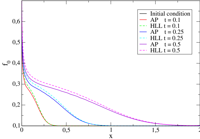
FIGURE 3. Hot wall: comparison of the temperature profile for the numerical solution (AP) and for the HLL scheme (HLL) at time 0.1, 0.25 and 0.5.
