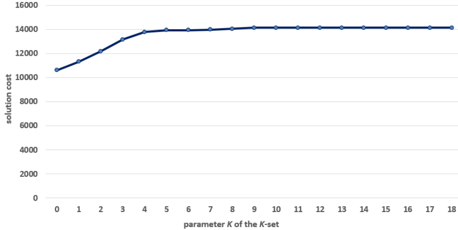
Figure 1: network pol ska – cost for different K -sets obtained with Algorithm 2 for continuous link capacities case (Phase 1).
