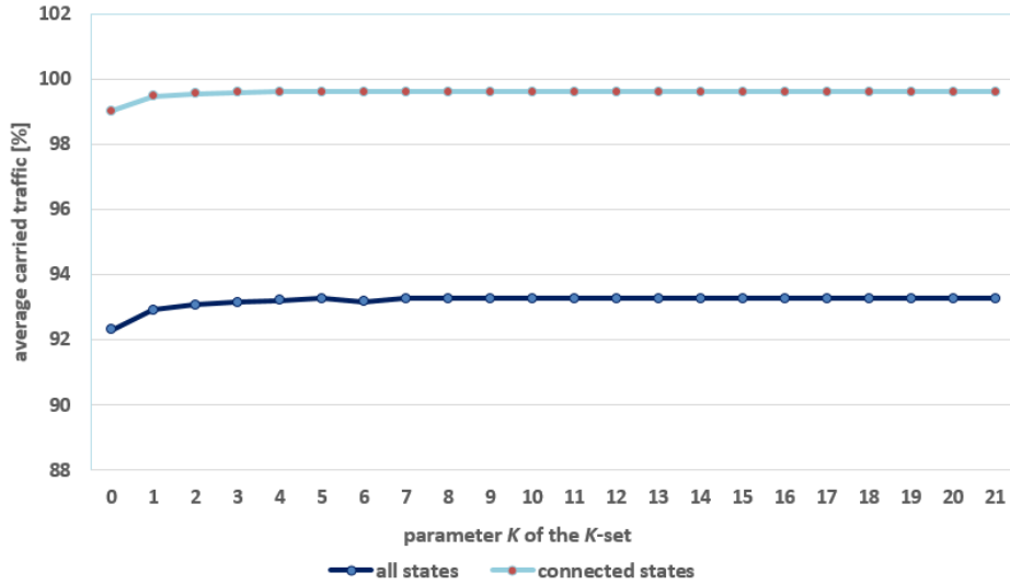
Figure 4: PMAN – states that are not covered with Algorithm 2.
