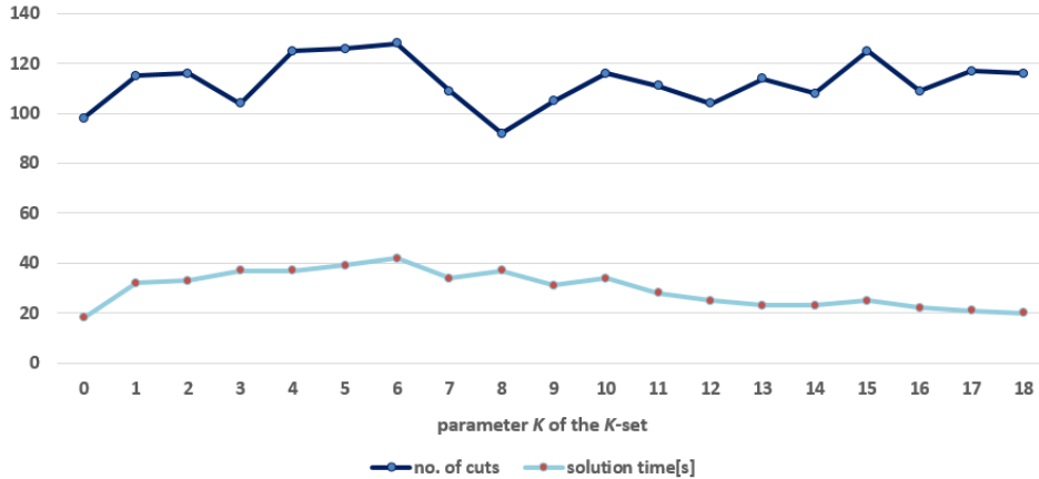
Figure 2: network pol ska – computation time and number of cuts achieved with Algorithm 2 for continuous link capacities case (Phase 1).
