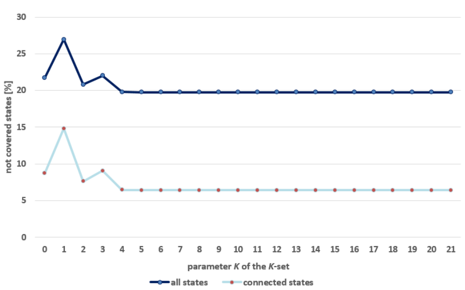
Figure 5: PMAN – results of robust optimization obtained with Algorithm 2.
