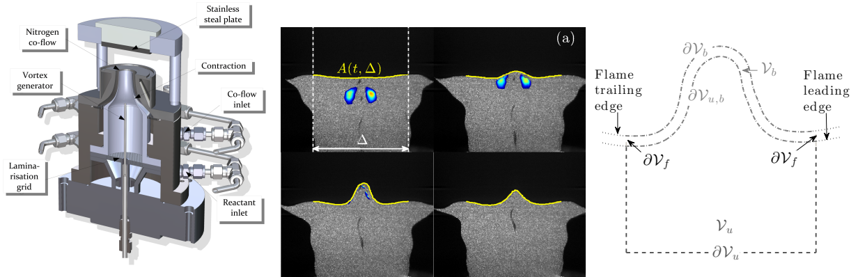
Figure 1: (left) Schematic of the Flame-Vortex Interaction Burner (FVIB). (center) Experimental contour of vorticity superimposed on the raw Mie scattering image together with the flame location. (right) control volume over which the fuel mass fraction is integrated to yield measurable expressions for the displacement and consumption speeds
