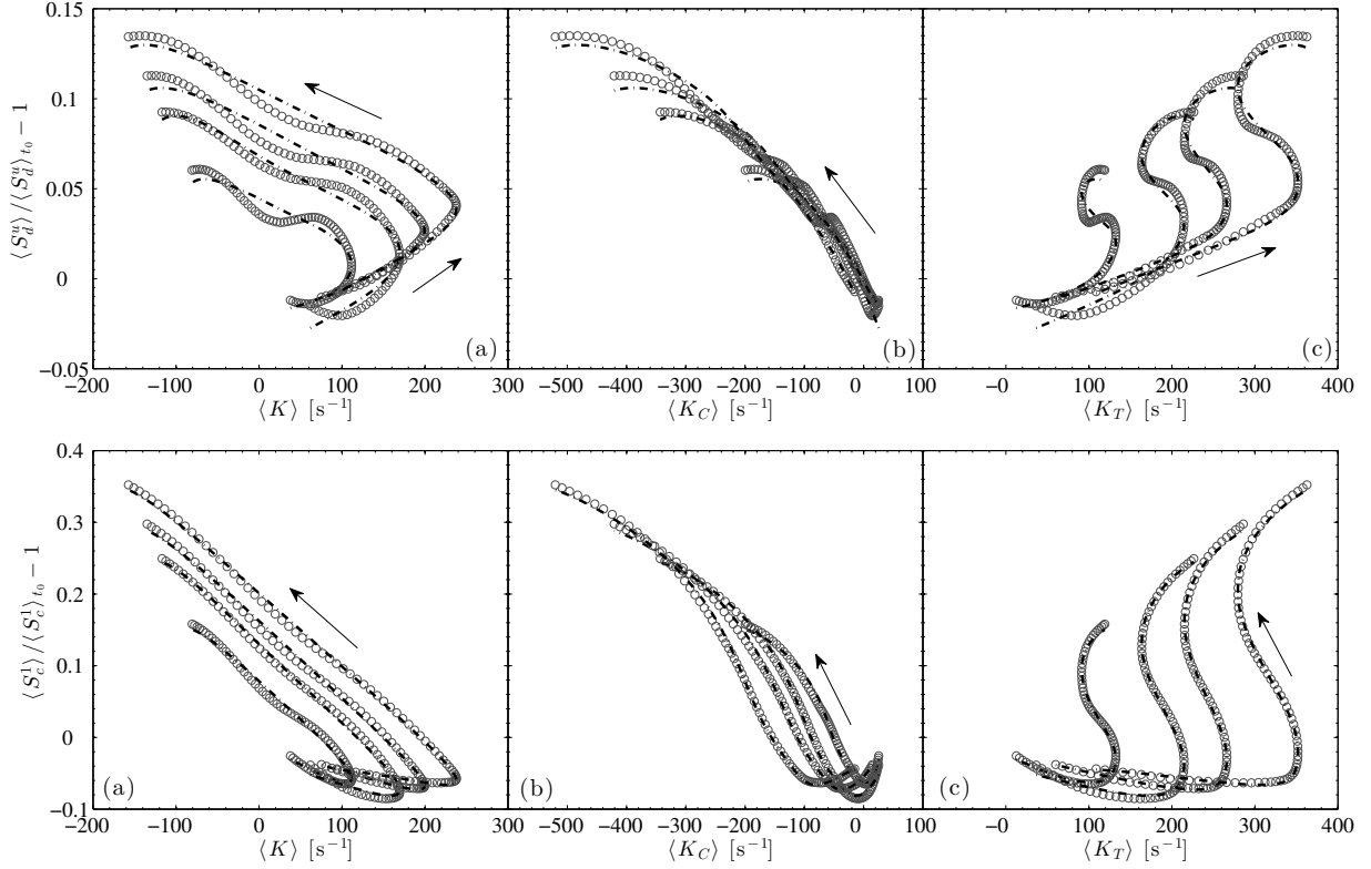
Figure 2: Plots of \langle S_d^u \rangle (top) and \langle S_c \rangle (bottom) versus \langle K \rangle (a), \langle K_C \rangle (b) and \langle K_T \rangle (c) for methane/air mixture at U_\theta / \langle S_c^1 \rangle_{t_0} = 2.8 . The arrow indicates the direction of increasing time. The different curves correspond to different width \Delta of the control volume; the smaller \Delta the larger the variations of \langle S_d^u \rangle , \langle S_c \rangle , \langle K \rangle , \langle K_C \rangle and \langle K_T \rangle . The dotted lines corresponds to predictions using Eqs. (5a) and (5b) with \mathcal{L}_\kappa = 4.98l_f and \mathcal{L}_K = -1.08l_f
