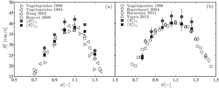
Figure 2: Comparison of the present assessment of the consumption speed for methane (a) and propane/air mixtures (b) at different equivalence ratios \phi with some data from the litterature. Error bars correspond to the standard deviation calculated from 15 independent measurements.
