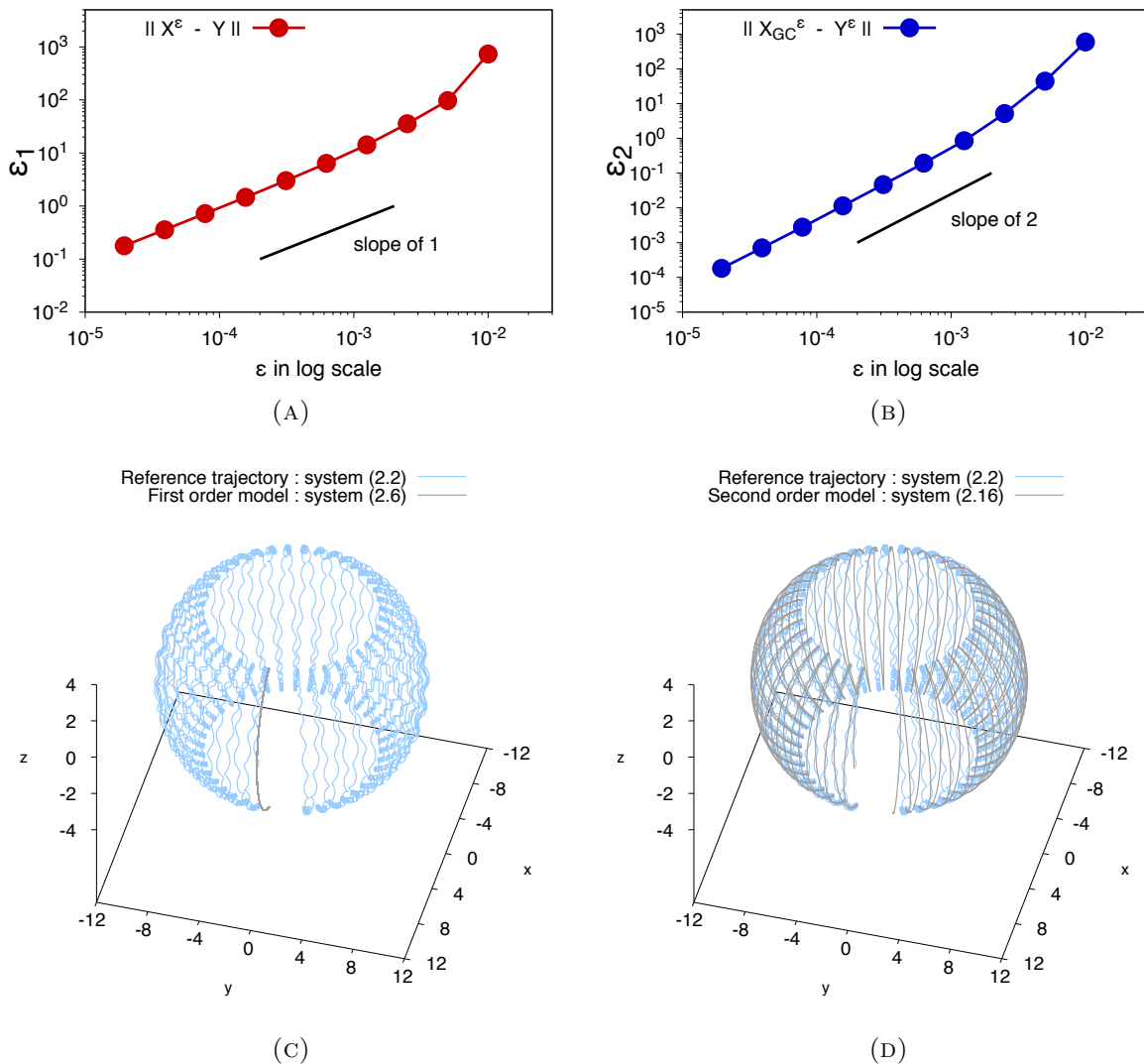
FIGURE 2. Numerical simulation: (A) error between the first order model and (2.2) (B) error between the second order model and (2.2) (C) particle trajectory obtained with the first order model and (2.2) (D) particle trajectory obtained with the second order model and (2.2).
