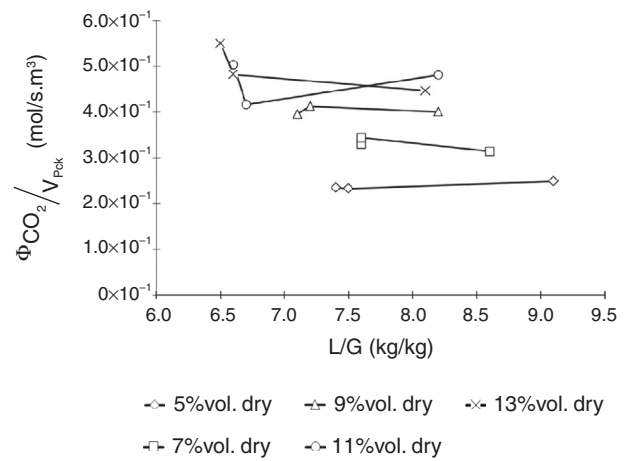
Figure 7 Absorption rate \Phi_{CO_2}/V_{pck} in function of CO 2 gas inlet for runs of experiment 1.
