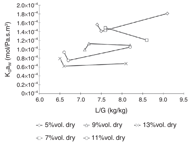
Figure 6 Overall mass transfer coefficient ( K_{GAW} ) in function of CO 2 gas inlet for runs of experiment 1.
