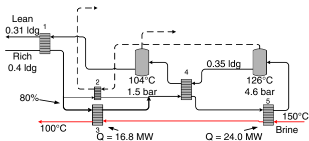
Figure 1 Advanced 2-Stage, 2-Pressure Flash (2T2Pflash) for amine solvent regeneration with geothermal brine heating.
