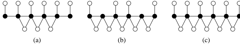
Fig. 2. Extremal cases where the lower bounds are attained, black vertices form a minimum (a) ID-code, (b) OLD-code, (c) LD-code.
