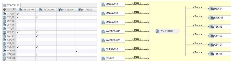
Fig. 4. Example: Traceability links among the tool set, framework and case study requirements
