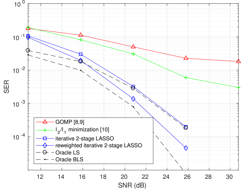
(a) BPSK with p_a = 15\%
