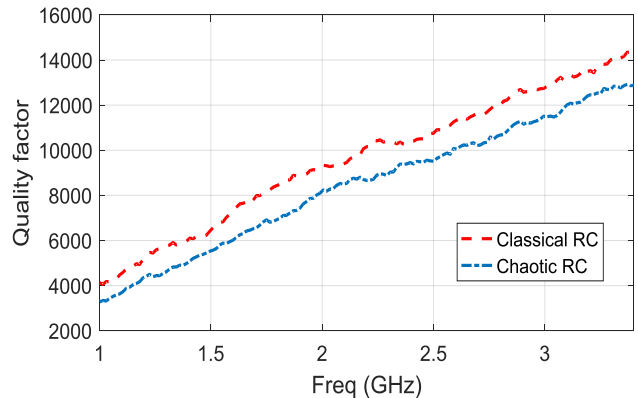
Fig. 7. Quality factors of the classical and the chaotic reverberation chambers.
