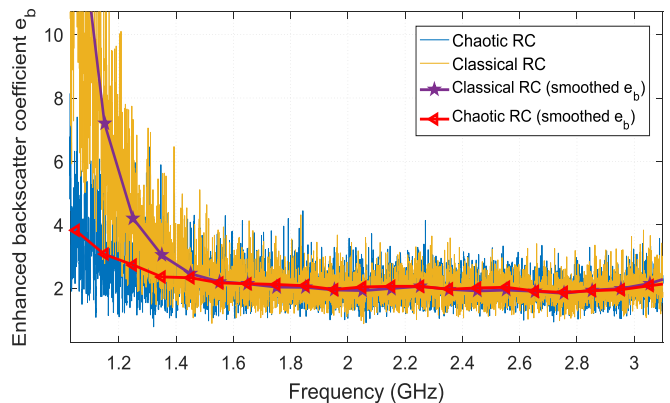
Fig. 8. Enhanced backscattering coefficient versus frequency in both RC configurations: classical and chaotic.
