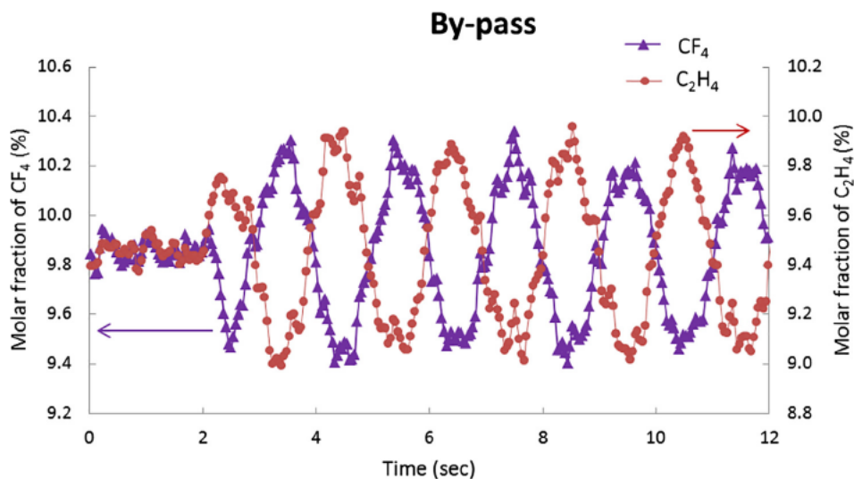
Fig. 9. Time-evolution of the molar fraction of \text{CF}_4 and \text{C}_2\text{H}_4 at the exit of the by-pass , for a frequency of 0.5 Hz and at ambient temperature. At first the catalyst is operated at steady-state conditions, then the oscillations are started (here at t \sim 2 s).
