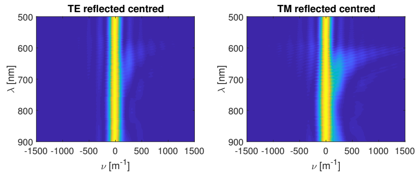
Fig. 16. TE and TM reflected beams after re-centering, for comparison to Fig. 15 (see text).
