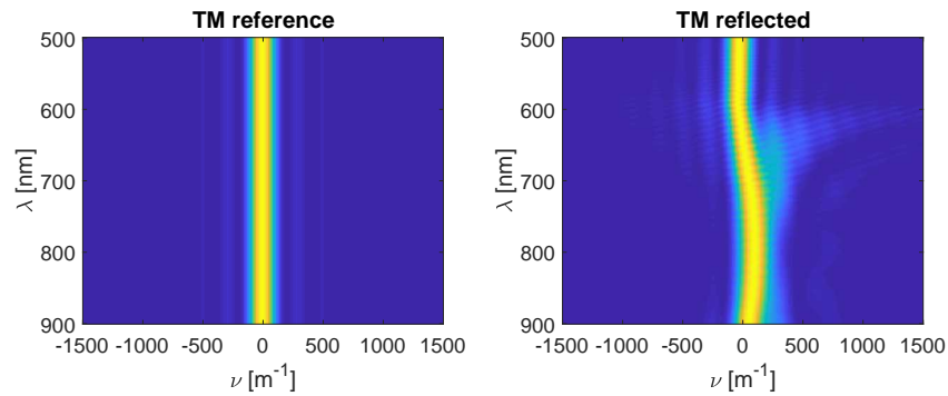
Fig. 15. TM reflected beam versus wavelength and spatial frequency. The left figure is the reference (see text) and the right figure emphasizes additional diffraction effects.
