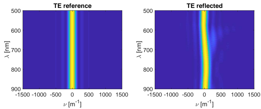
Fig. 14. TE reflected beam versus wavelength and spatial frequency. The left figure is the reference (see text) and the right figure emphasizes additional diffraction effects.
