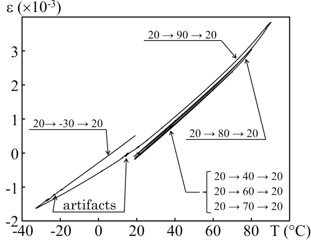
Figure 5: Thermal longitudinal strain \epsilon versus temperature T under cyclic thermal loading between ambient and the glass transition temperature. The first three cycles (up to 70^\circ\text{C} ) are superimposed, reversible, and virtually indistinguishable.
