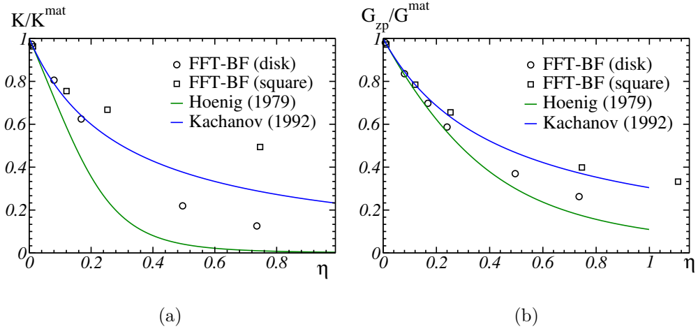
Figure 13: Normalized effective bulk modulus \tilde{K}/K^{\text{mat}} (a) and shear modulus G_{zp}/G^{\text{mat}} (b), of a random array of parallel cracks for increasing crack density \eta . The cracks have a cylindrical shape of width w = 1 voxel and either circular (black disks) or square cross section (black squares). Solid lines: homogenization theories for a matrix containing a random set of parallel elliptical cracks. Blue: “non-interacting” approximation ( Kachanov, 1992 ); Green: estimate of Hoenig (1979) .
