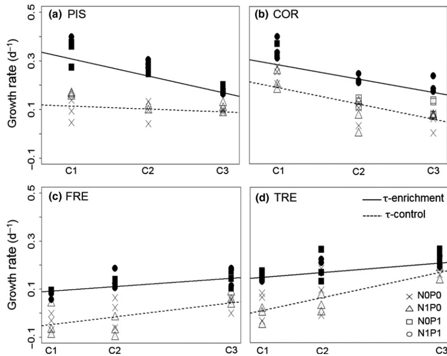
FIGURE 5 Linear regression between phytoplankton growth rates in microcosms and sampling time during the ice-free period, according to the two types of nutrient conditions ( \tau -control in dotted line and \tau -enrichment in limiting nutrients in solid line). Results are presented for each lake, for each sampling campaign represented as the number of days since the first day of sampling (C1, C2 and C3) and for the four initial microcosm nutrient enrichments (no addition—N0P0, N addition—N1P0, P addition—N0P1, N plus P addition—N1P1). White symbols are for the microcosms attached to the \tau -control category and black symbols for the \tau -enrichment category
