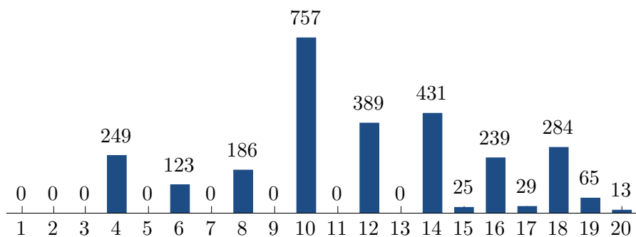
Figure 7.2. Occurrence of each possible values of the Picard number in the dataset
