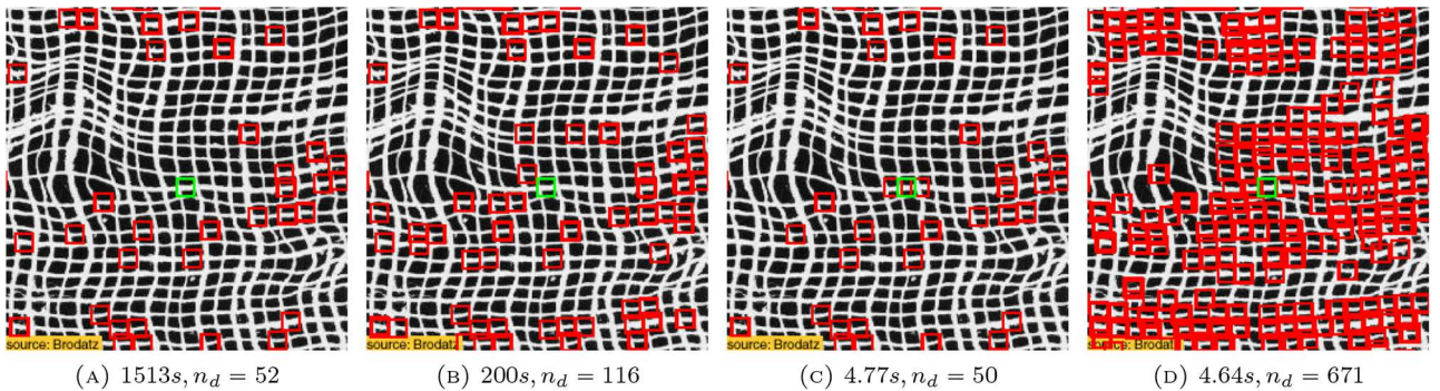
FIGURE 9. Similarity detection. In this figure we illustrate the accuracy of the different proposed approximations of the cumulative distribution function of \mathcal{AS}_{2,2}(U, \mathbf{t}, \omega) . We say that an offset \mathbf{t} is detected in an image if \mathcal{AS}_{2,2}(u, \mathbf{t}, \omega) \leq a(\mathbf{t}) for some threshold a(\mathbf{t}) \in \mathbb{R} . In every image, in green we display the patch domain \omega (in the center of the image) and in red we display the shifted patch domain for detected offsets with function a(\mathbf{t}) such that for any \mathbf{t} \in \Omega , \mathbb{P}[\mathcal{AS}_{2,2}(U, \mathbf{t}, \omega) \leq a(\mathbf{t})] = 1/256^2 , where U is given by the Gaussian random field f * W where f is the original image of fabric and W is a Gaussian white noise over \Omega = 256 \times 256 . Approximations of the cumulative distribution function of \mathcal{AS}_{2,2}(U, \mathbf{t}, \omega) lead to approximations of a(\mathbf{t}) . The most precise approximation is given in (A) where the eigenvalues are computed using a MATLAB routine and the cumulative distribution function is given by the Imhof method. In (B) we approximate the eigenvalues using the projection described in Proposition 4.2 and still use the Imhof method. It yields twice as many detections. In (C) Wood F method is used instead of Imhof's yielding less detections but performing seven times faster. Interestingly errors seem to compensate and the obtained result with Wood F method is very close to the results obtained with the baseline algorithm in (A). In (D) HBE method is used instead of Imhof's, in this case we obtain too many detections, i.e. the approximation of the cumulative distribution function is not valid.
