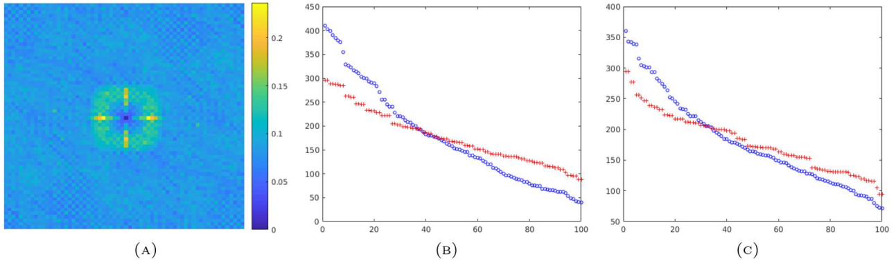
FIGURE 7. Eigenvalues approximation. We consider a Gaussian random field generated with f * W with W a Gaussian white noise and f is a fixed sample of an independent Gaussian white noise over \Omega . We consider patches of size 10 \times 10 and study the approximation of the eigenvalues for the covariance matrix of the random field restricted to a domain of size 10 \times 10 , similarly to Proposition 4.1. (A) shows the Normalized Root-Mean Square Deviation between the eigenvalues computed with standard routines and the ones given by the approximation for each offset, see (4.2). Offset zero is at the center of the image. (B) and (C) illustrate the properties of Proposition 4.2. Blue circles correspond to the 100 eigenvalues computed with MATLAB routine for offset (5, 5) in (B), respectively (10, 20) in (C), and red crosses correspond to the 100 approximated eigenvalues for the same offsets. Note that a standard routine takes 273s for 10 \times 10 patches on 256 \times 256 images whereas it only takes 1.11s when approximating the eigenvalues using the discrete Fourier transform.
