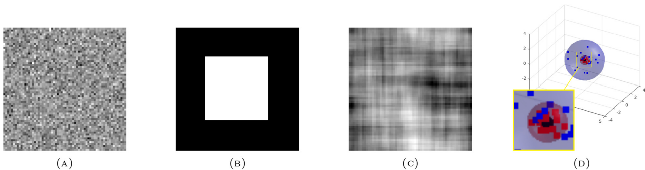
FIGURE 2. Gaussian models and spatial redundancy. In this experiment we illustrate the notion of spatial redundancy in two models. In (A), we present a 64 \times 64 Gaussian white noise. (B) Shows an indicator function f . In (C), we present a realization of the Gaussian random field defined by f * W (with periodic convolution) where W is a Gaussian white noise over \Omega (domain of size 64 \times 64 ). Note that f was chosen so that the two Gaussian random fields (A) and (C) have the same gray-level distribution for each pixel. To each pixel position in (A) and (C) we associate the surrounding patch, with patch domain \omega (of size 3 \times 3 ). Hence, for each image (A) and (C) we obtain 64 \times 64 = 5096 vectors each of size 3 \times 3 = 9 . These 9-dimensional vectors are projected in a 3-dimensional space using Principal Component Analysis. In the subfigure (D), we display the 20 vectors closest to 0 in each case: Gaussian white noise model (in blue) and the Gaussian random field (C) (in red). The radius of the blue, respectively red, sphere represents the maximal L^2 norm of these 20 vectors in the Gaussian white noise model, respectively in model (C). Since the radius of the blue sphere is larger than the red one the points are more scattered in the patch space of (A) than in the patch space of (B). This implies that there is more spatial redundancy in (C) than in (A), which is expected.
