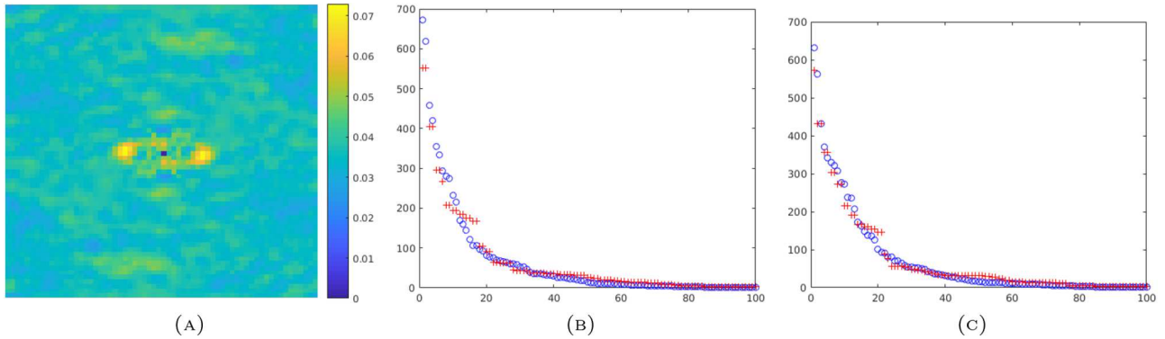
FIGURE 8. Eigenvalues approximation. Same study as the one conducted in Figure 7 with f = \mathbb{1}_{\{1,2,3\}^2} . Note that in this case the approximation is better than the one presented in Figure 7.
