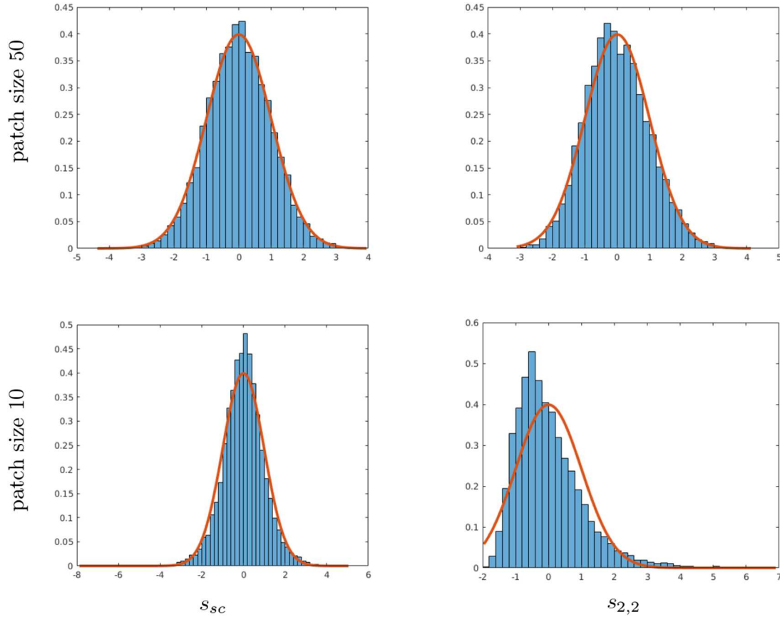
FIGURE 5. Gaussian moment matching. In this experiment, 10^4 samples of 128 \times 128 Gaussian images are computed with a spot of size 5 \times 5 (the spot is the indicator of this square). Scalar product auto-similarities and squared L^2 auto-similarities are computed for a fixed offset (70, 100) . We then plot the normalized histogram of these values. The red curve corresponds to the standard Gaussian \mathcal{N}(0, 1) . On the top row r = 100 \gg 1 and the Gaussian approximation is valid. On the bottom row r \approx 1 and the Gaussian approximation is not valid.
