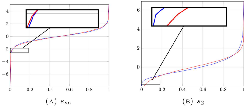
FIGURE 6. Theoretical and empirical cumulative distribution Function. This experiment illustrates the non-Gaussianity in Figure 5. In both cases, the red curve is the inverse cumulative distribution function of the standard Gaussian and the blue curve is the empirical inverse cumulative distribution function of normalized auto-similarity functions computed with 10^4 samples of Gaussian models. We present auto-similarity results obtained for \mathbf{t} = (70, 100) and similarity function s_{sc} (on the left) and s_2 (on the right). We note that for rare events, see the magnified region, the theoretical inverse cumulative distribution function is above the empirical inverse cumulative distribution function. The opposite behavior is observed for similarity s_2 . These observations are in accordance with the findings of Table 1.
