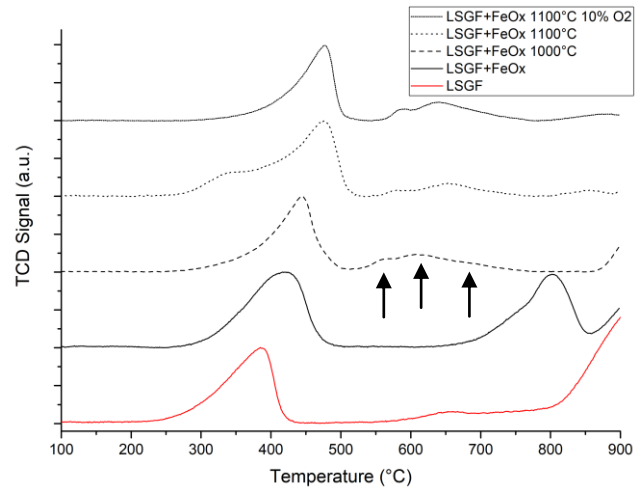
Figure 6. TPR profiles of LSGF + FeO x treated at different temperatures. In red, the profile of LSGF before the deposition is shown for comparison.
