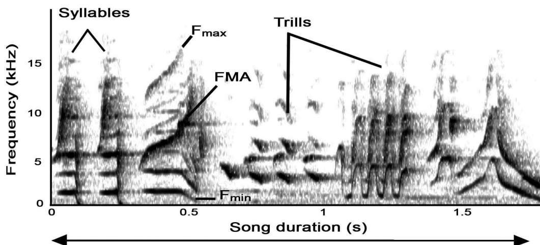
Figure 2. A spectrogram of the long-range song of a mainland male tūi ( Prothemadera novaeseelandiae ), showing the variables employed in this study.
