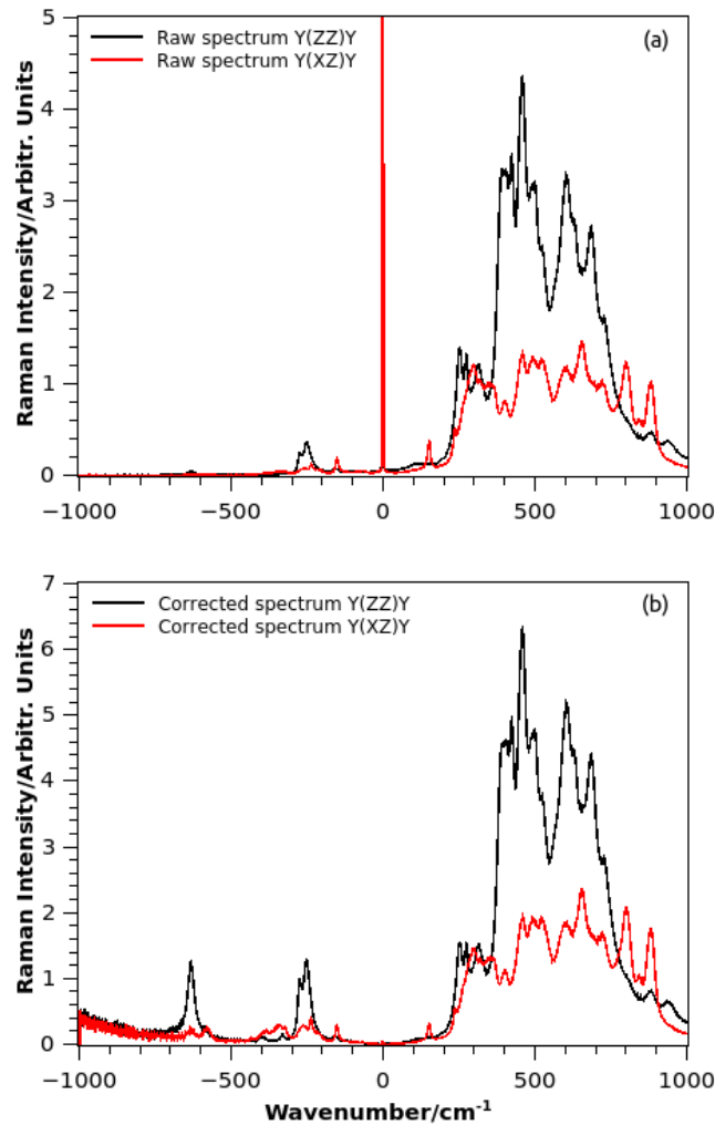
Figure 4. Spectra recorded on 1% mol Ho 3+ -doped LN in Y(ZZ)Y and Y(XZ)Y configurations. (a) raw data; (b) spectra after corrections.
