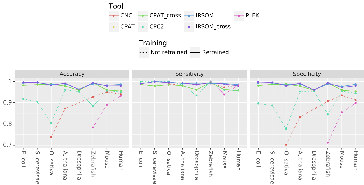
Figure 2: Accuracy results obtained by CNC2, CNCI, CPAT, PLEK and IRSOM on each of Human, Mouse, A. thaliana thaliana , Oryza saliva , Zebrafish, Escherichia coli , Saccharomyces cerevisiae and Drosophila species. CPAT_cross and IRSOM_cross designate respectively CPAT and IRSOM when used with the cross-species model. CPAT and IRSOM are by default used on each species with the corresponding model. Two models for CNCI are available, one for vertebrate and one for plants. CPC2 was trained on Human protein and ncRNA in GENCODE. And PLEK was trained on Human data.
