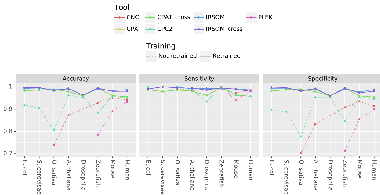
Figure 2: Accuracy results obtained by CNC2, CNCI, CPAT, PLEK and IRSOM on each of Human, Mouse, A. thaliana thaliana , Oryza saliva , Zebrafish, Escherichia coli , Saccharomyces cerevisiae and Drosophila species. CPAT_cross and IRSOM_cross designate respectively CPAT and IRSOM when used with the cross-species model. CPAT and IRSOM are by default used on each species with the corresponding model. Two models for CNCI are available, one for vertebrate and one for plants. CPC2 was trained on Human protein and ncRNA in GENCODE. And PLEK was trained on Human data.
