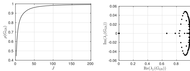
FIGURE 5. Left: Spectral radius of the AltMR as a function of the number of objects. Right: Example of the spectrum of the (one-dimensional) operator G_{GS} = -(D + L)^{-1}U . Notice that many eigenvalues are clustered around 1.
