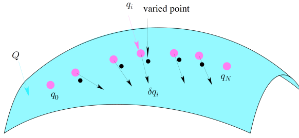
Fig. 1 The discrete form of Hamilton's principle (Lew et al. 2003).
