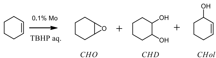
Scheme 3. Epoxidation of cyclohexene.
