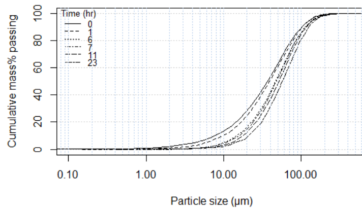
Fig. 7. Predicted rate of change of Ni-slag PSD during the mineralization process ( T=150^{\circ}\text{C} , P_{\text{CO}_2}=20\text{ atm} )
