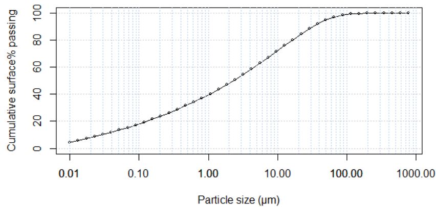
Fig. 2. Typical particle size distribution of Ni-slags for the mineralization process
