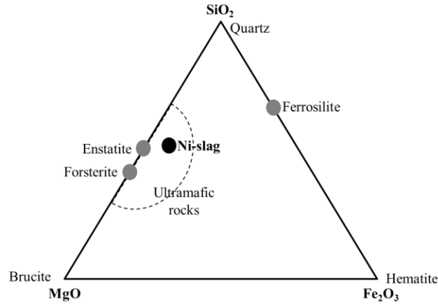
Fig. 1. Position of New Caledonian Ni-slags in the \text{MgO-Fe}_2\text{O}_3\text{-SiO}_2 composition diagram
