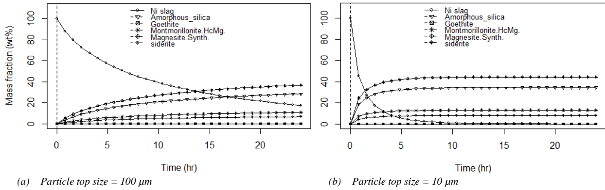
Fig. 6. Predicted mineralization product phases ( T=150^{\circ}\text{C} , P_{\text{CO}_2}=20\text{ atm} ).
