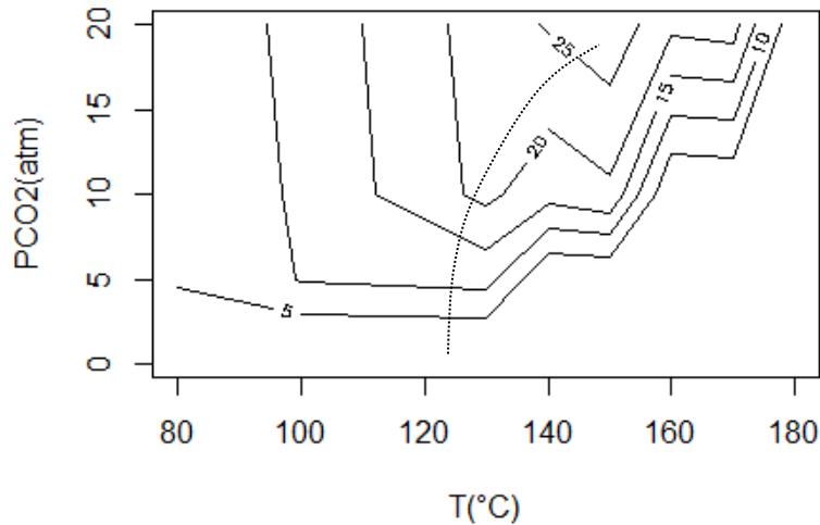
Fig. 5. Predicted mass percent of amorphous silica in mineralization product as a function of temperature and P_{CO_2}
