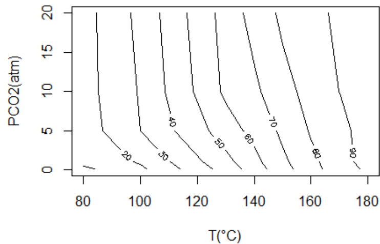
Fig. 3. Predicted Ni-slag dissolution extent as a function of temperature and P_{\text{CO}_2}
