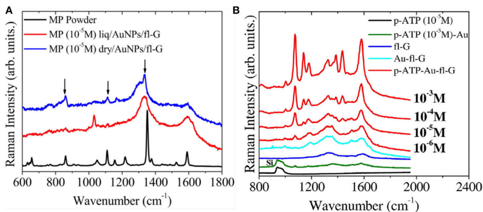
FIGURE 14 | (A) Raman spectra at 633 nm of methyl parathion (MP) on Au-fl-G concentrated at 10 -5 M and 10 -4 M at liquid and dry states. (B) Raman spectra at 633 nm of p-ATP(10 -5 M) on Si, p-ATP(10 -5 M) on AuNPs deposited on Si, fl-graphene, AuNPs/fl-G, and p-ATP on AuNPs/fl-G at different p-ATP concentration (10 -6 M, 10 -5 M, 10 -4 M, 10 -3 M) [Reproduced from Tite et al. (2016) with permission of Elsevier].
