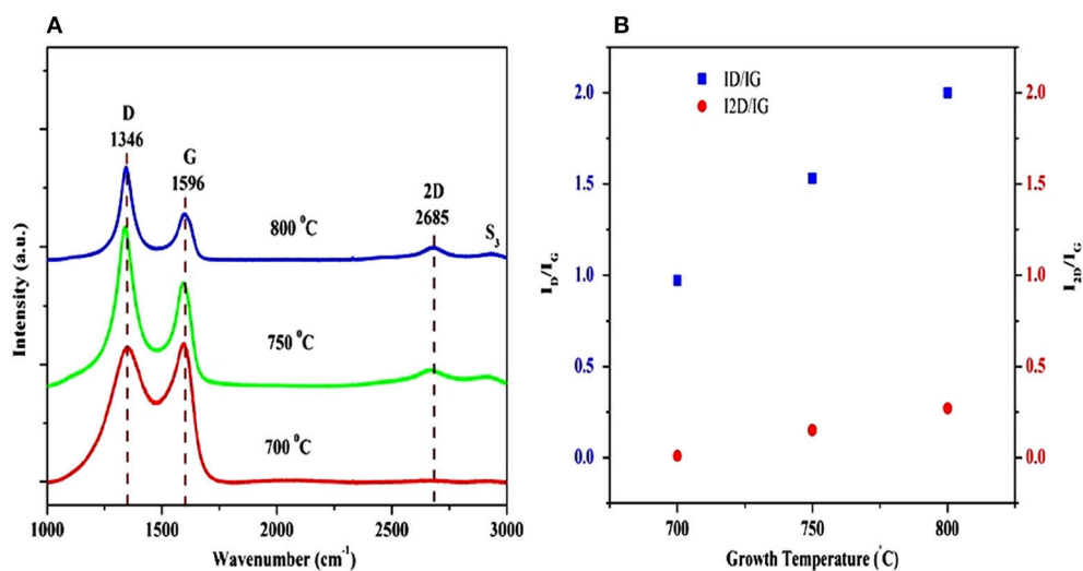
FIGURE 11 | (A) Raman spectra of graphene films deposited on Ni/Si substrate at three different growth temperatures; (B) I_D/I_G and I_{2D}/I_G intensity ratios of graphene layers as a function of the growth temperature [Reproduced from Kumar et al. (2017) with permission of Springer]. (B) shows the I_D/I_G and I_{2D}/I_G ratios as a function of growth temperature. Clearly, the intensity ratios I_D/I_G and I_{2D}/I_G increased with the increase in growth temperature. The I_{2D}/I_G ratio for the graphene film deposited at 750°C was 0.15, confirming the formation of multi-layer graphene (7–8 layers). The I_{2D}/I_G ratio for graphene films grown at 800°C was 0.27, corresponding to few-layer graphene (4–5 layers).
