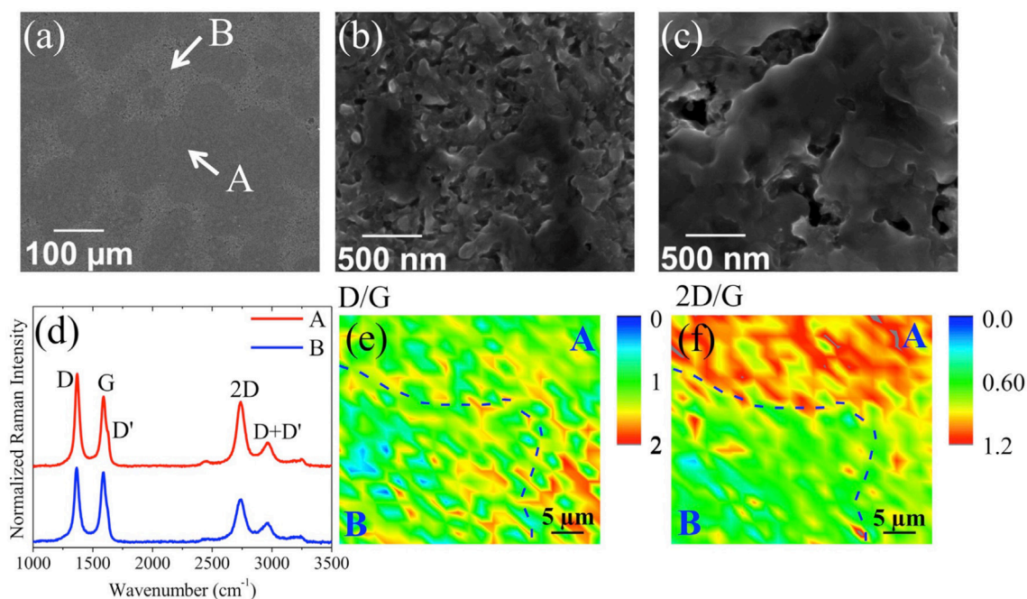
FIGURE 10 | SEM images of a-C (5 nm)/Ni/Si after thermal processing at (a) 500 × and 12,000 × magnifications for the areas A (b) and B (c) showing a 3D porous structure; (d) typical Raman spectra at 442 nm taken in regions A and B. Raman mapping at 442 nm of the intensity ratio on 40 μm × 40 μm of (e) D/G and (f) 2D/G, respectively. The dashed lines are guides delimiting regions A and B [Reproduced from Tite et al. (2016) with permission of Elsevier].
