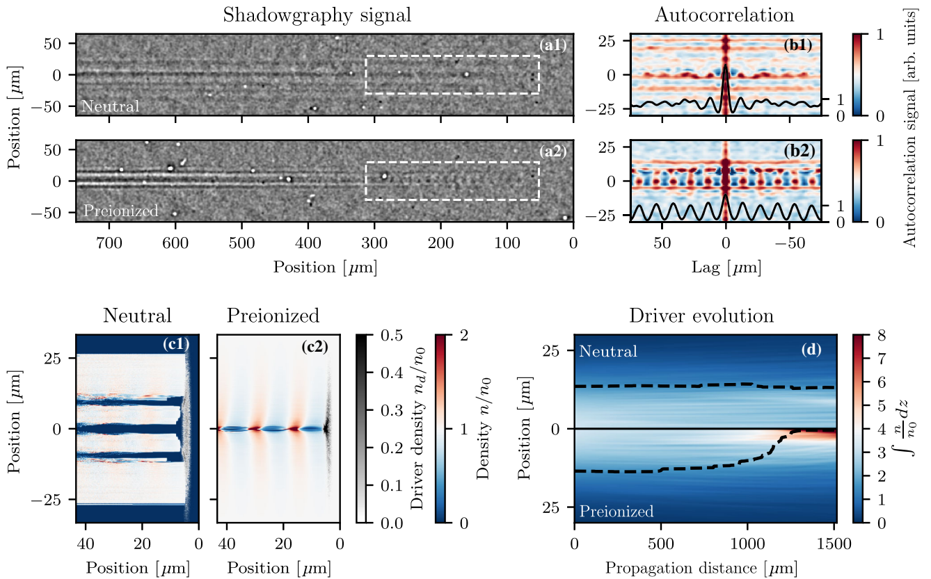
FIG. 3. Electron-driven plasma waves with blocked laser. Top : (a) Shadowgrams of the second jet for neutral and preionized hydrogen gas. The drive bunch propagates from left to right. (b) Row-wise autocorrelations within the region of interest (dashed rectangle). The graphs in (b) are the horizontal lineouts at vertical zero. The transverse modulation in the neutral case can only be attributed to ionization from the electron beam. The autocorrelation (b1) shows no indication of a longitudinal signal modulation that would be generated by a plasma wave. However, the preionized case (a2) shows a weak, but visible periodical longitudinal modulation which is caused by a plasma wave driven by the electron beam. This modulation is clearly visible in the autocorrelation (b2). Bottom : Full 3D simulations of the interaction. (c) Charge densities of the background plasma electrons (blue-red color scale) along with the driver (gray color scale). The regions in (c1) where the electron density is zero correspond to nonionized gas. (d) Evolution of the transverse (longitudinally integrated) driver density for both cases, along with their half width at half maximum (HWHM, dashed line). The driver in the preionized case self-focuses much faster and drives a stronger plasma wave, even with full blowout of the background electrons. In the neutral case the driver is not able to fully ionize the gas. See Fig. S3 in the Supplemental Material [47] for a close-up of the drivers.
