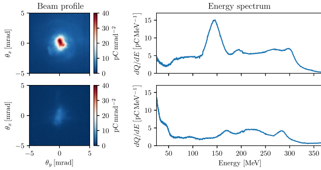
FIG. 5. Beam profile and energy spectra of representative shots with only the first gas jet (top) and with tape and second gas jet (bottom).
