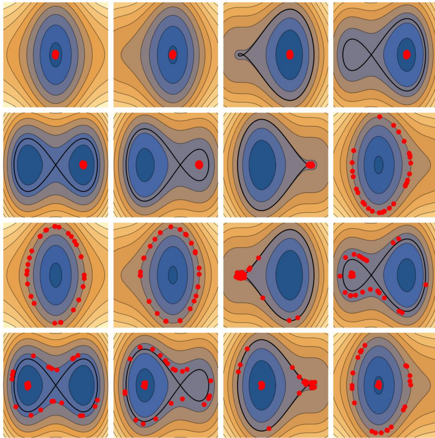
FIG. 2: Separation in energy reached by abrupt separation of orbits. Frames show snapshots at increasing times (from left to right and from top to bottom) of the phase-space (x, p) position of a bunch of particles (red dots). The contour levels are those of H_1(t) (Eq. 2) with \phi = \pi/2 . Particles are initialized close to the origin; they stay grouped together until the lobe disappears (7th frame); then distribute along the iso-energy level. After the lobe and the separatrix reappear (11th frame), particles are separated into two distinct groups, one with the original energy, and another with a higher energy.
