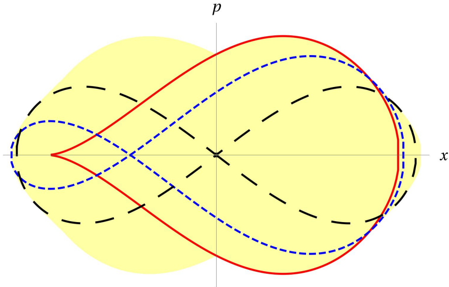
FIG. 1: Snapshots of the slowly pulsating separatrix. The three curves represent the separatrix at different times. Red solid curve, the separatrix is just appearing with a single right lobe; blue short-dashed curve, a left lobe is developing; black long-dashed curve, the two lobes are symmetrical with respect to the p axis; during the next half-period, the separatrix evolves with mirror symmetry. The yellow domain is the total area swept by the separatrix throughout one period. The figure has been produced with A = 3 .
