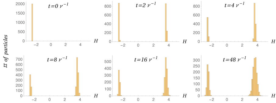
FIG. 4: Histogram of the energy distribution at different times. We bin the energy of a set of 2000 particles initially almost at rest ( x, p \approx 0 ), with A = 3, \omega = 0.003 . All the simulations were run for a fixed phase of the wave such that particles are initially close to the O-point. Another example, for a different value of the phase, is reported in the Fig. S2 in the file Supplementary Figures online.
