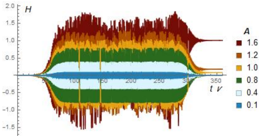
FIG. 3: Particle energy H_1 vs. time. Several values of the amplitude A are considered. Only in the cases A \geq 1 there is a net gain in the final particle energy. These results have been obtained at a fixed phase of the wave; by varying the phase, the final value of H_1 may change at most by 30%.
