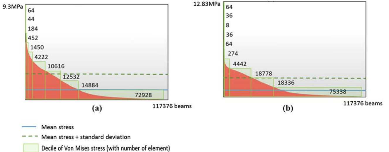
Fig. 11 Initial A criterion for both classic and stretched lattice structures (Fig. 7), von Mises stress value per element sorted form highest to lowest. a Uniform lattice, b non-uniform lattice
