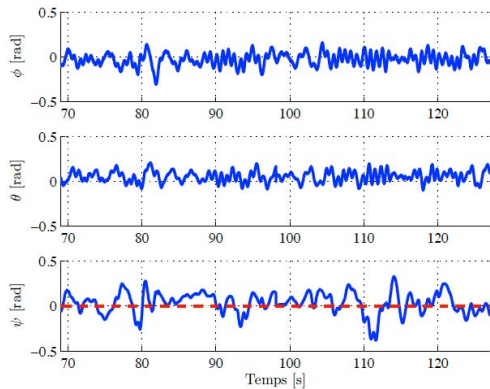
Fig. 27. Experimental test: response of Euler angles (solid line) and their references (dashed line) measured with the preliminary prototype.
