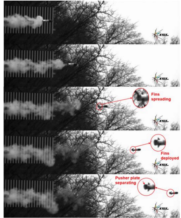
Fig. 5. Beginning of the GLMAV ballistic flight.
