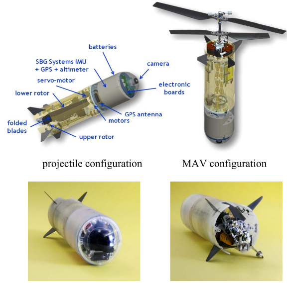
Fig. 1. Final version 2.0 of the GLMAV platform.
