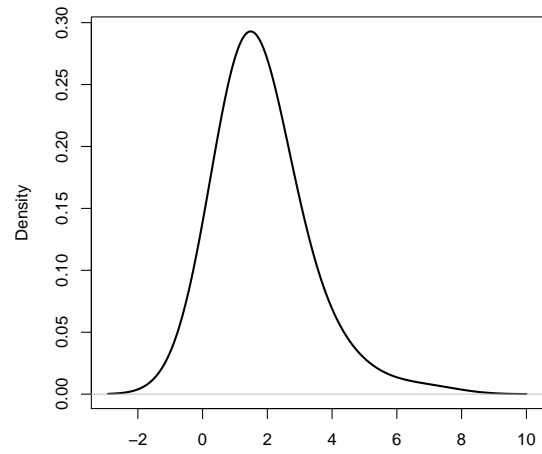
Figure 4: Kernel density plots for the considered data set.
