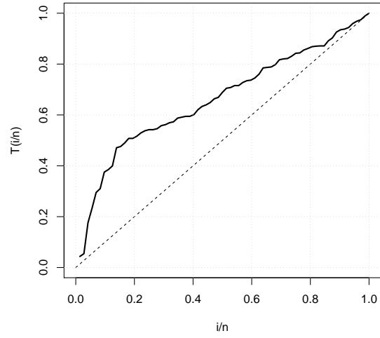
Figure 3: TTT plots for the considered data set.
