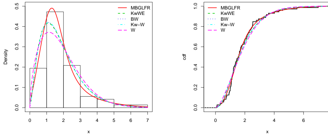
Figure 5: Plots of estimated pdfs and cdfs for given data set.
